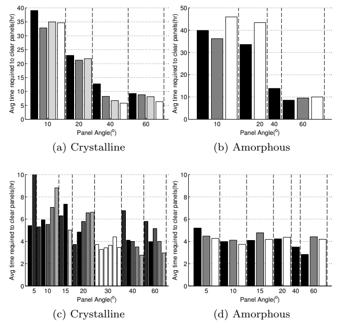
Figure 7: Mean time to clear for c-Si, (a) and (c) and a-Si:H, (b) and (d) for the winter of 2010/2011 (a),(c) and 2011/2012 (b),(d) respectively. The colour of the bar represents a module from a specific manufacturer
