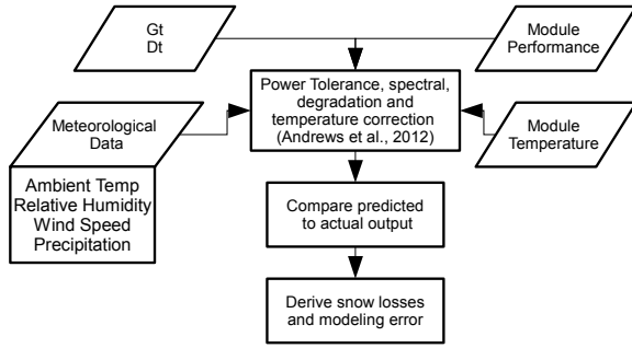
Figure 2: Data processing flowchart, G_t and D_t represent the time series of measured global and diffuse irradiance respectively. Module performance in this case is defined as a timeseries of I_{sc} .
